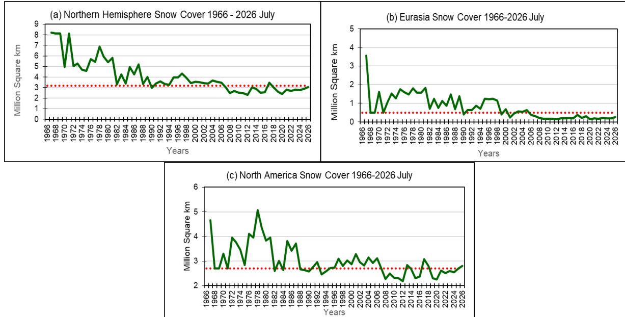
Fig 5: Snow cover area (million Sq. km) for the month of July during the period 1966-2026 (green solid lines) and normal value (1991-2020) (red dotted line) for (a) Northern Hemisphere (b) Eurasia and (c) North America. (Data Source: Rutgers University Snow Lab).
