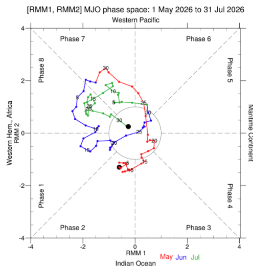
Fig.6. RMM phase diagram for Madden Julian Oscillation (MJO) for the period May to July 2026. (Data Source: http://www.bom.gov.au/climate/mjo/ ).
