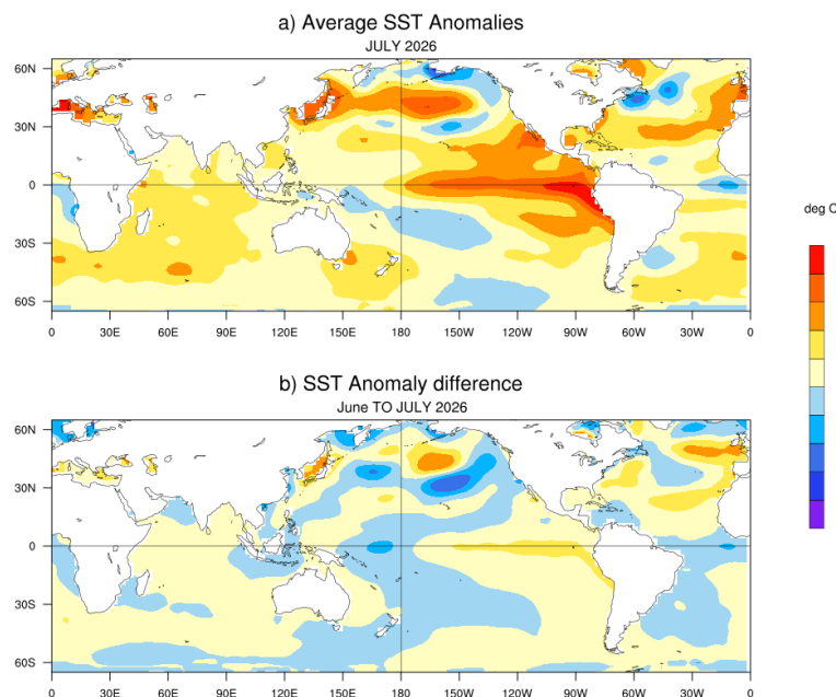
Fig.1: (a) Sea surface temperature (SST) anomalies ( ^{\circ}\text{C} ) during July 2026 and (b) changes in the SST anomalies ( ^{\circ}\text{C} ) from June to July 2026. SSTs are based on the ERSSTv5, from NOAA, and anomalies are computed with respect to 30-year (1991-2020) long term mean.
