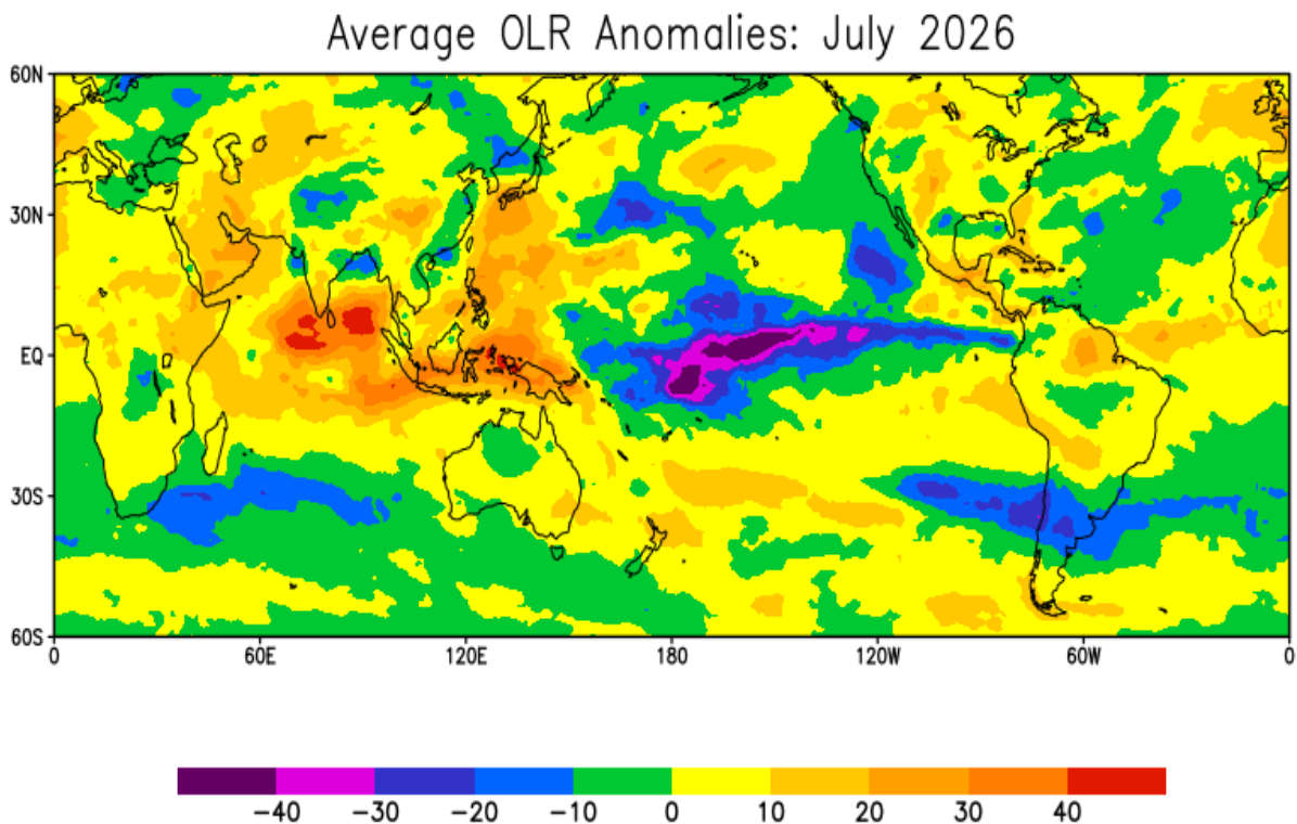
Fig.4: Outgoing Long Wave Radiation (OLR) Anomaly ( \text{W/m}^2 ) for July 2026 (Data source: NCEP-NOAA)
