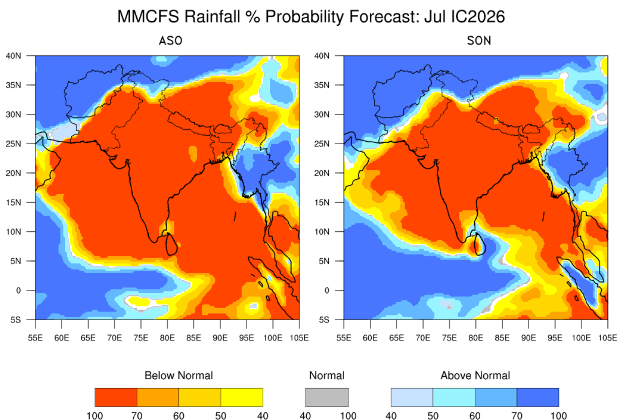
Fig.7: Seasonal probability (%) forecasts of precipitation for (a) ASO 2026 (left) and (b) SON 2026 (right) based on initial conditions of July 2026. The white colour indicates climatological probability.
