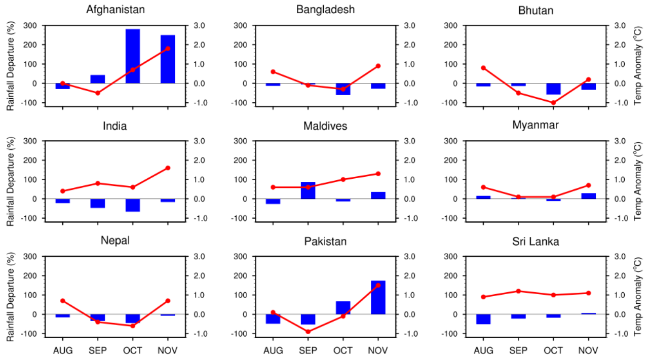
Fig. 9: Monthly country averaged rainfall forecast expressed as percentage departures (%) and monthly country averaged temperature anomaly (°C) forecast during August to November 2026. Here, the normal range for country averaged monthly precipitation is taken as -10% to +10% (Left Vertical Axis Scale for Precipitation indicated in blue shaded bars) and the normal range for country averaged monthly temperature is taken -0.25°C to +0.25°C (Right Vertical Axis Scale for Temperature indicated in red colored lines).
