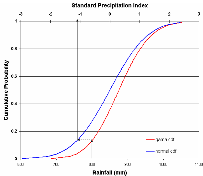
Fig.3. Illustration of computation of SPI for the seasonal rainfall over the country as a whole obtained through equiprobability transformation from fitted gamma cumulative probability distribution to standard normal cumulative probability distribution. The southwest monsoon season rainfall over the country as a whole for the period 1901-2003 was used to fit the gamma distribution. For a rainfall value of 800mm the transformation provides SPI value of -1.1118.
